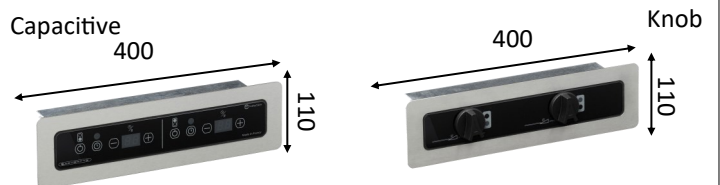
Control cut out dimensions 370 x 72mm
