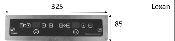
Control cut out dimensions 302 x 60mm
